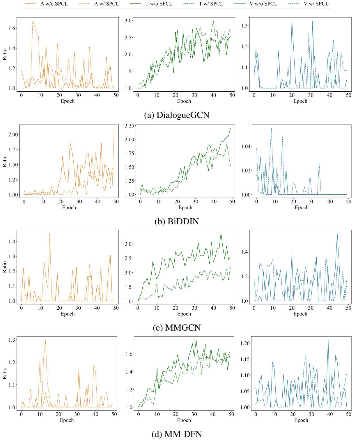
Figure 4.11: Modality ratio of the four backbones during training on IEMOCAP dataset.
