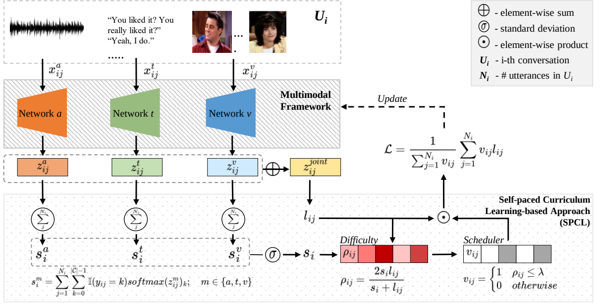
Figure 4.8: Our framework pipeline with integrated SPCL module.
