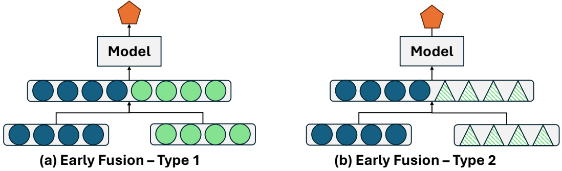
Figure 1.3: Classical multimodal fusion strategies: Early fusion
