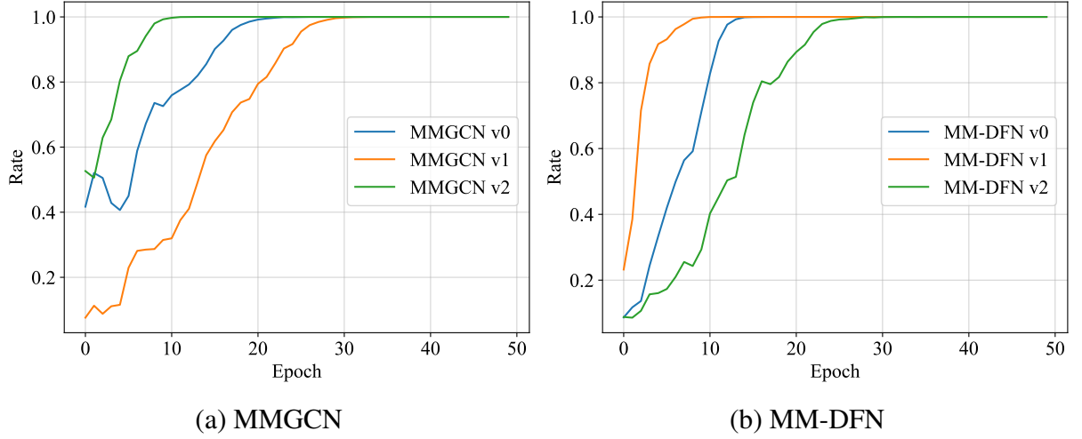
Figure 4.10: Curricula expanding rate of MMGCN and MM-DFN under SPCL hyper-parameters setting specified in Table 4.8.
