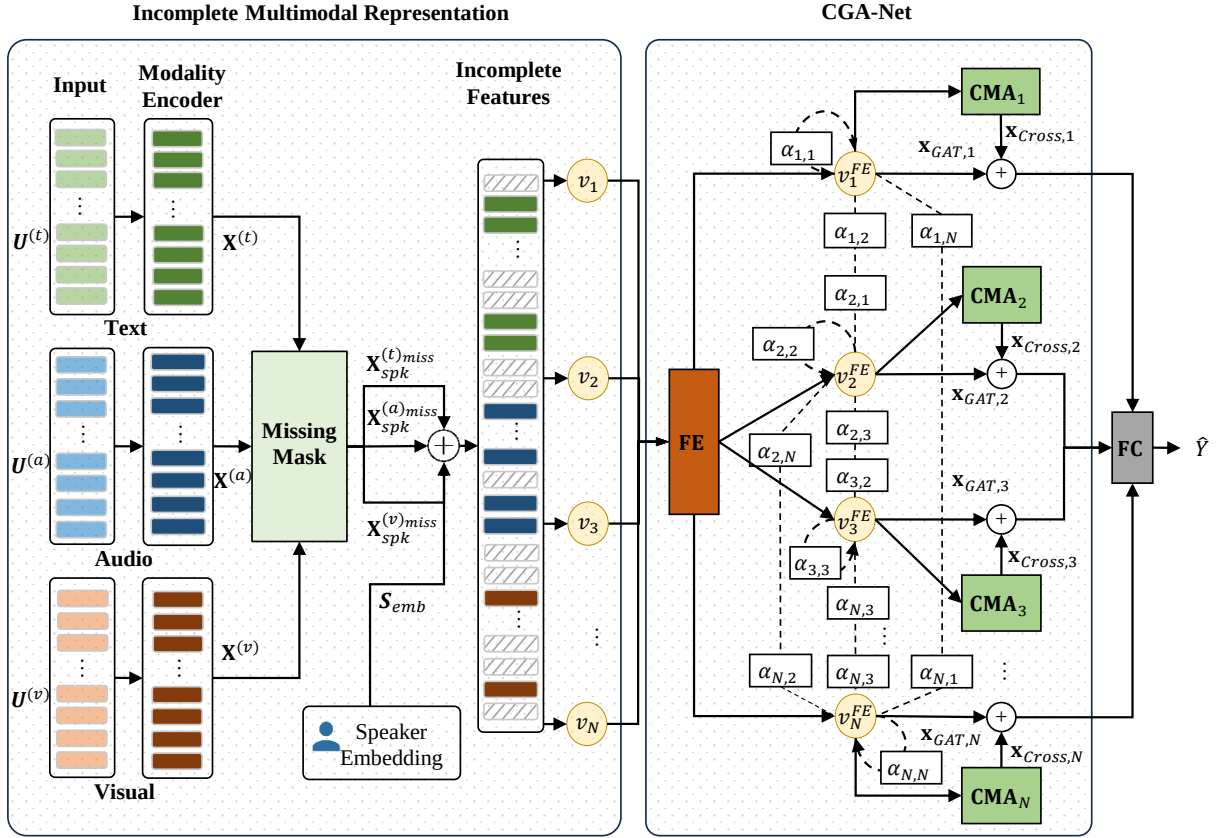
Figure 3.2: Overall Architecture of Mi-CGA model.
