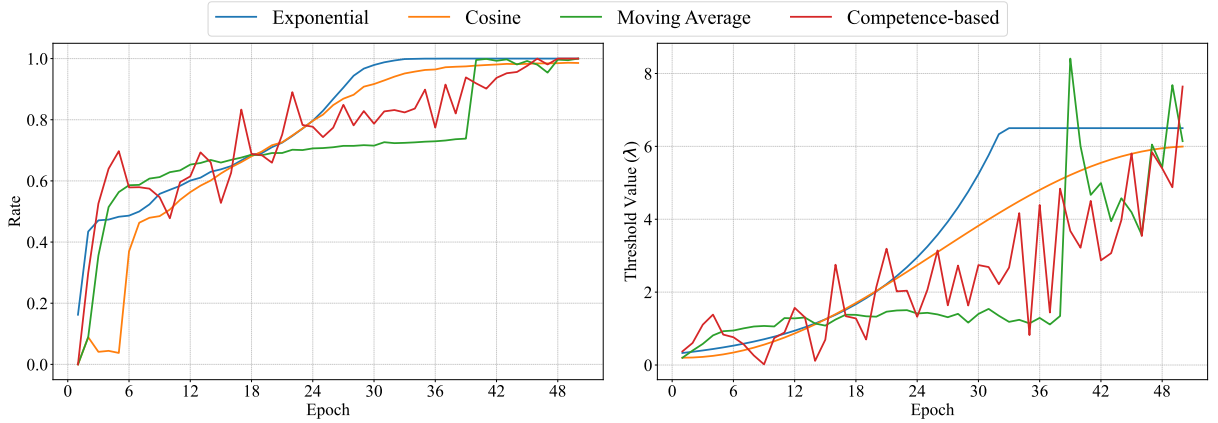
Figure 4.12: Curricula expanding rate and respective threshold value of MMGCN on MELD under different pacing strategies.
