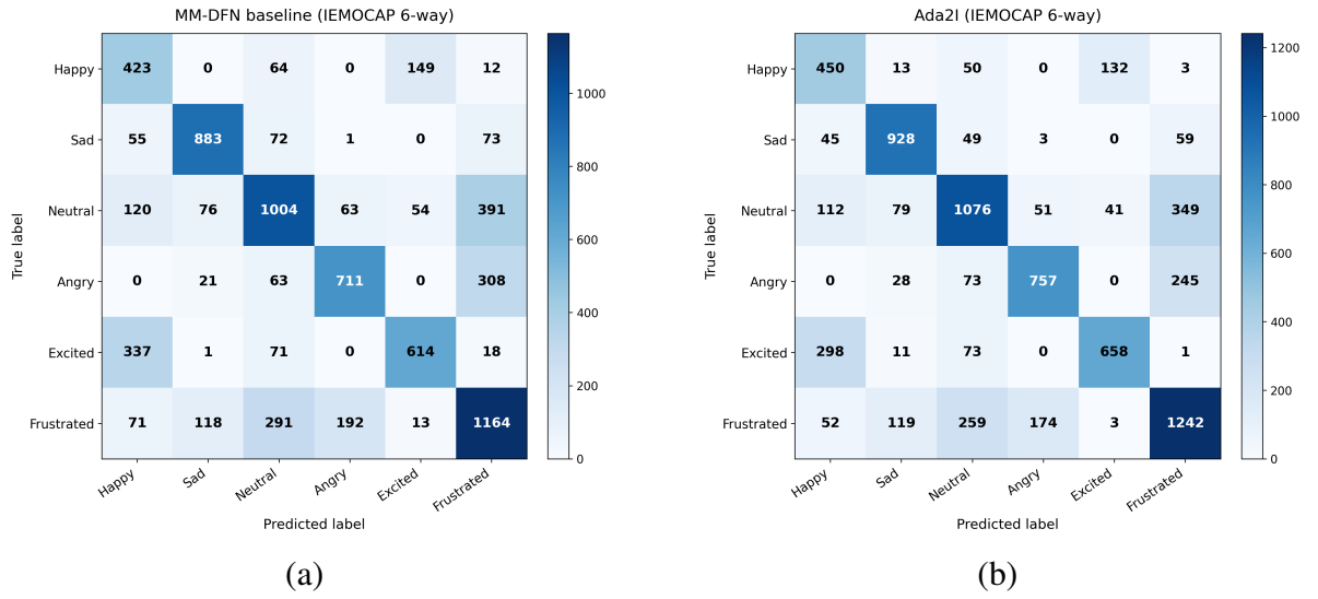
Figure 4.5: Confusion matrices on the IEMOCAP 6-way dataset for (a) the baseline MM-DFN model and (b) the proposed Ada2I model.
