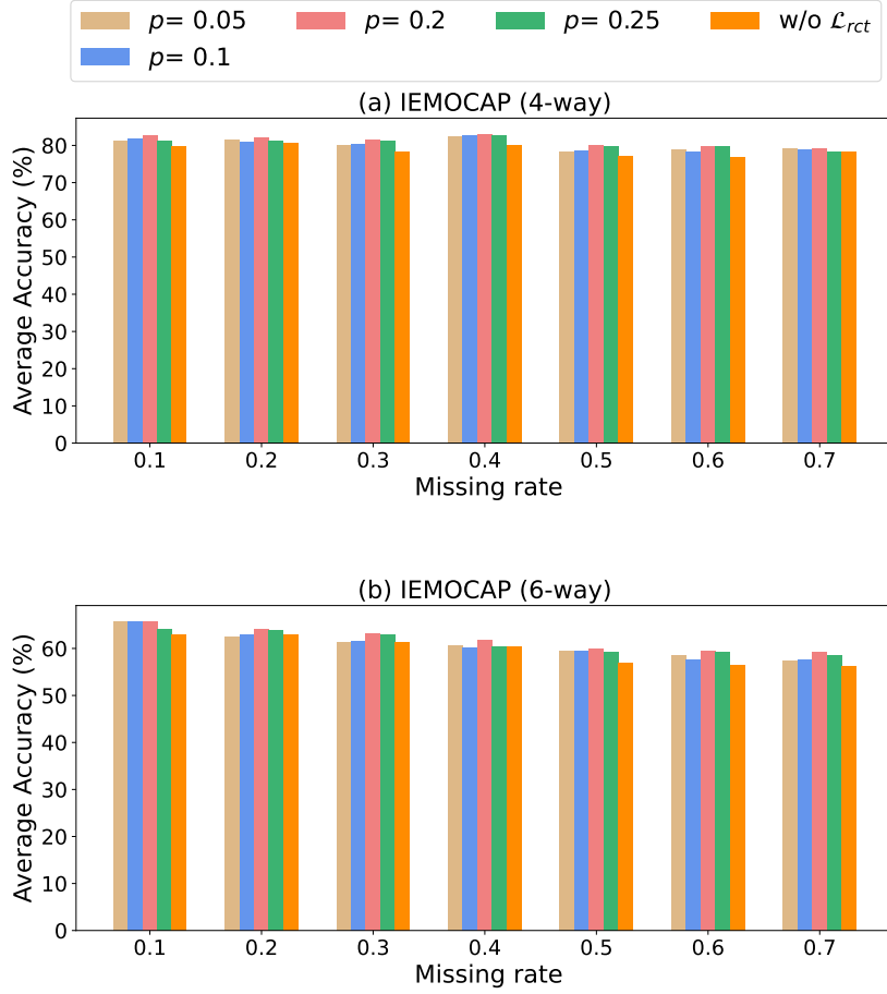
Figure 3.9: A comparison of the impact of the p value in \mathcal{L}_{rct} . The default setting in Mi-CGA is p = 0.2 . The results for different p values show minimal variation, but they consistently outperform the scenario without \mathcal{L}_{rct} .
