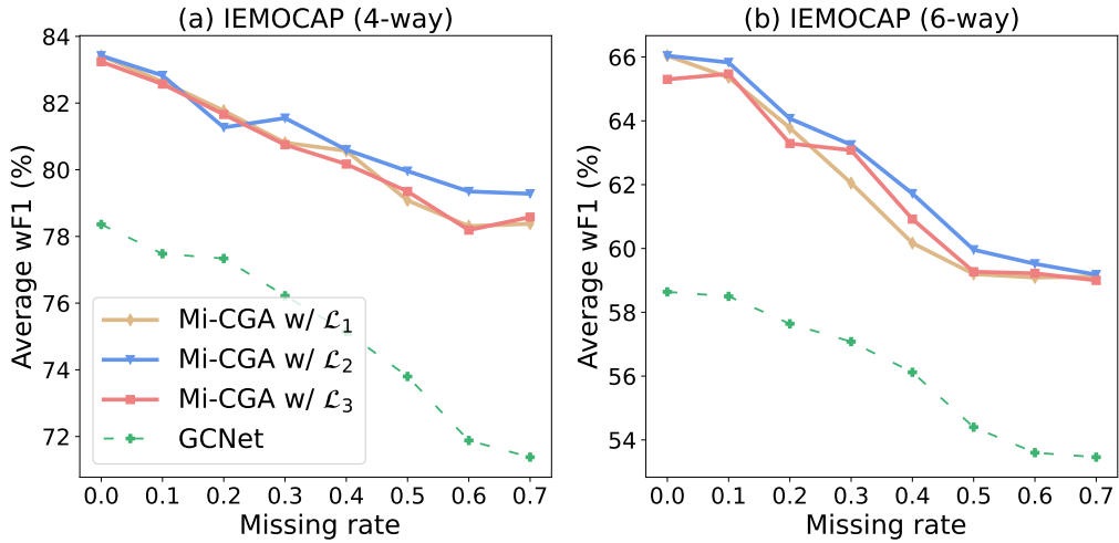
Figure 3.8: Illustration of our Mi-CGA performance with different types of objective function on IEMOCAP datasets.
