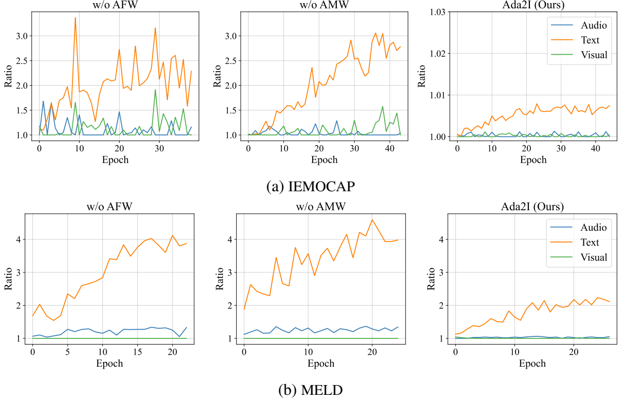
Figure 4.6: The change of the discrepancy ratio \rho^t, \rho^a, \rho^v on the IEMOCAP and MELD datasets during training, along with various ablation tests including without AMW and without AFW, are compared to the Ada2I model.
