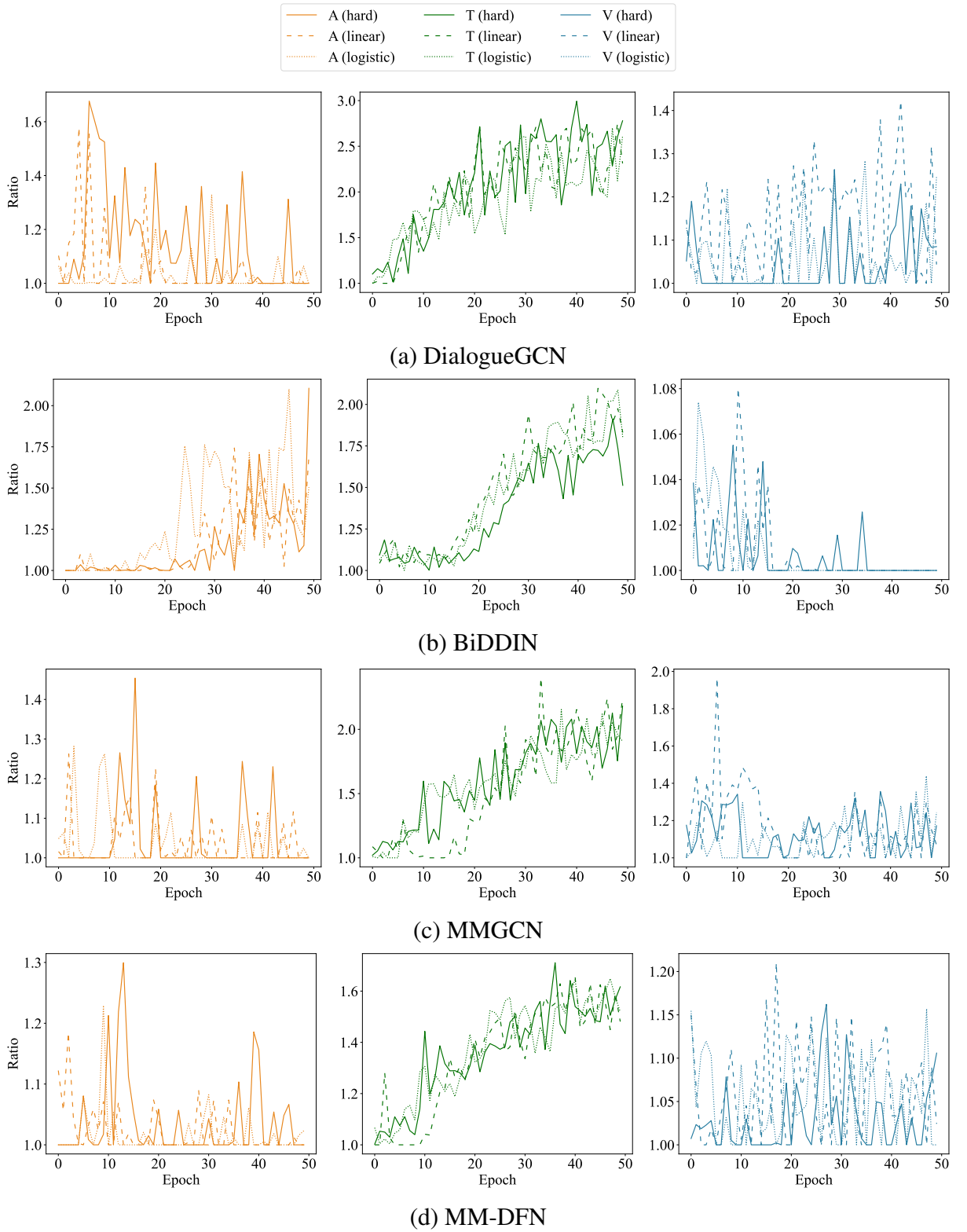
Figure 4.13: Modality ratio of the four backbones during training on IEMOCAP dataset using different types of regularizer for the Learning Scheduler.
