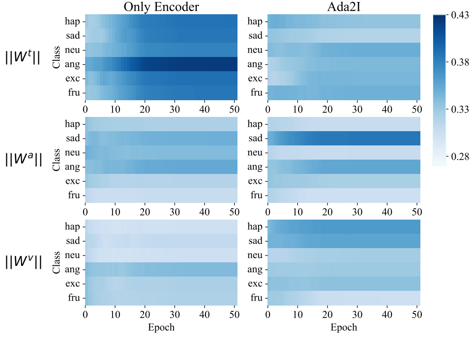
Figure 4.7: Modality-wise weights of each label normalized for the IEMOCAP dataset
