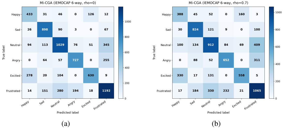
Figure 3.6: Illustrative confusion matrices of Mi-CGA on the IEMOCAP 6-way dataset under (a) complete-modality conditions ( \rho = 0 ) and (b) severe modality incompleteness ( \rho = 0.7 ).
