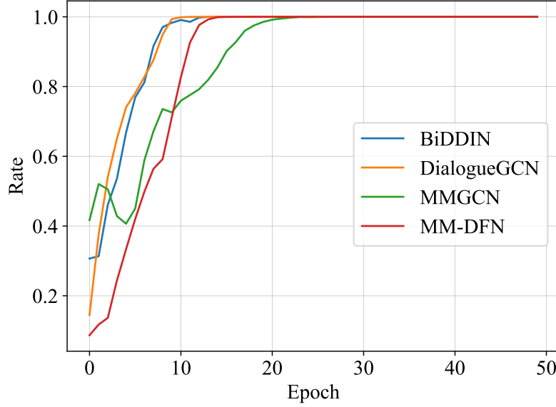
Figure 4.9: The curricula expanding rate of the four baselines integrated on IEMOCAP.
