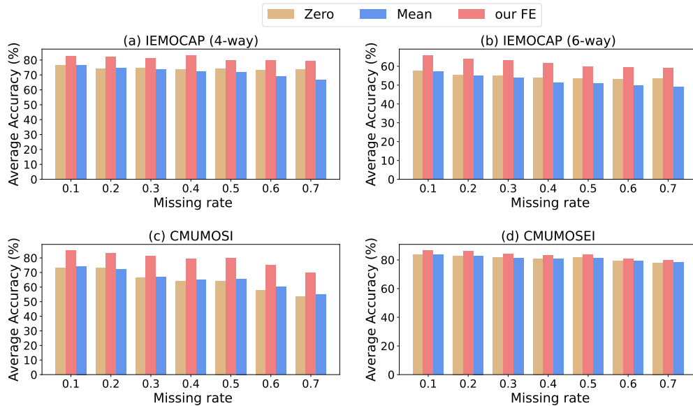
Figure 3.7: Illustration of the robustness in performance of our proposed feature estimation against basis approaches in the different rate of missing in modalities.
